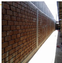
Standard Soil Interlocking Block (200mm x 115mmx100mm)
